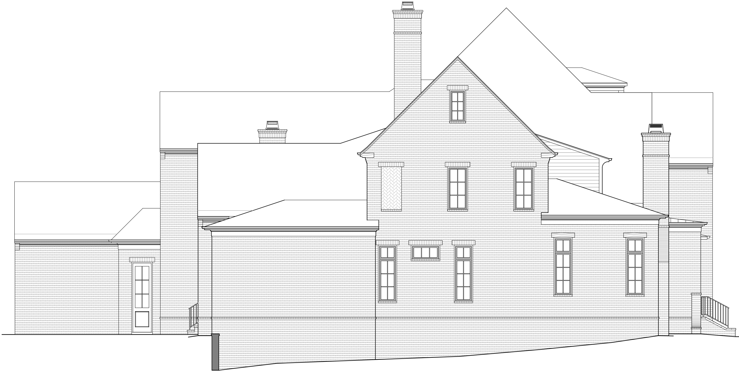
1 LEFT ELEVATION 1/4" = 1'-0"
