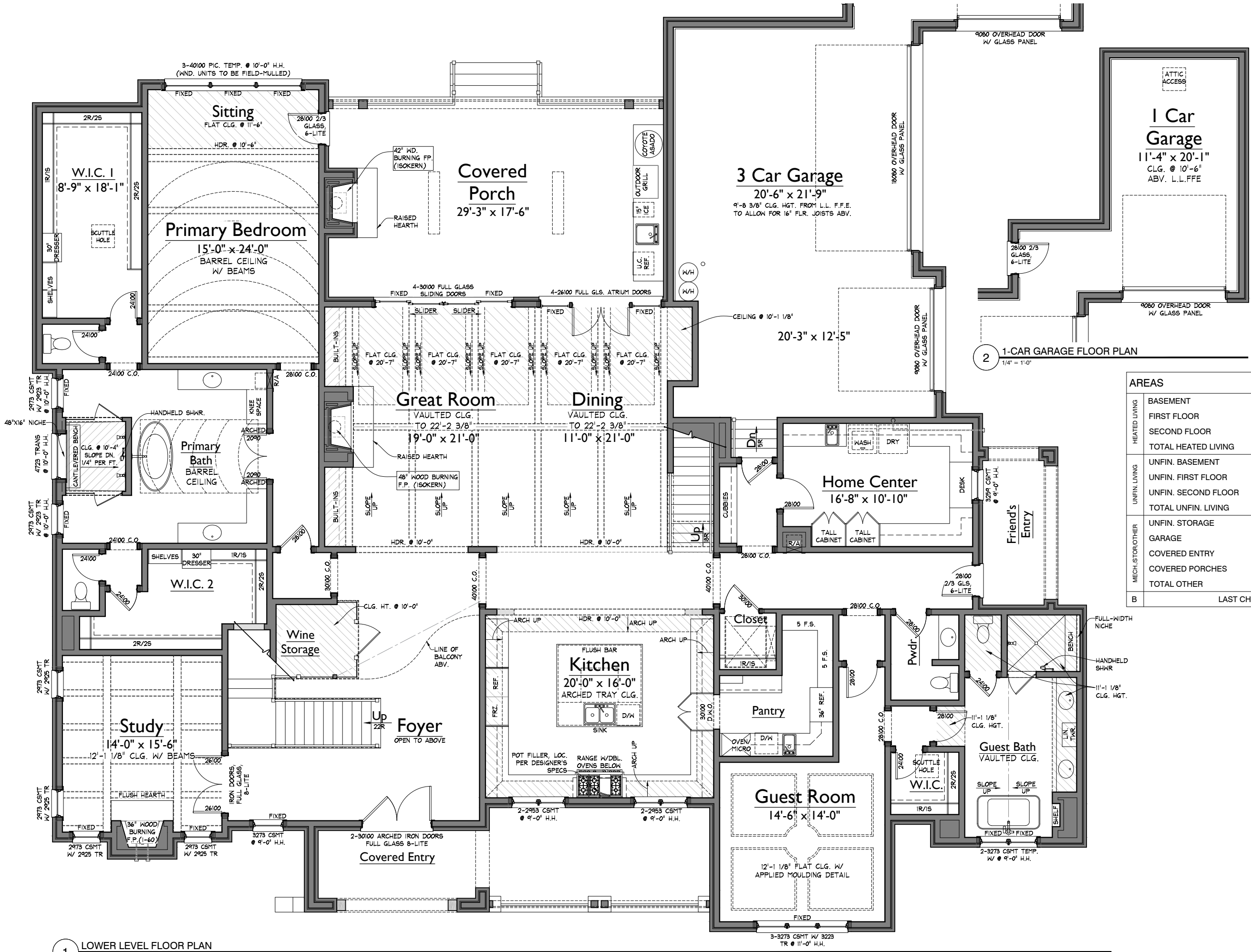
1 LOWER LEVEL FLOOR PLAN 1/4" = 1'-0"
