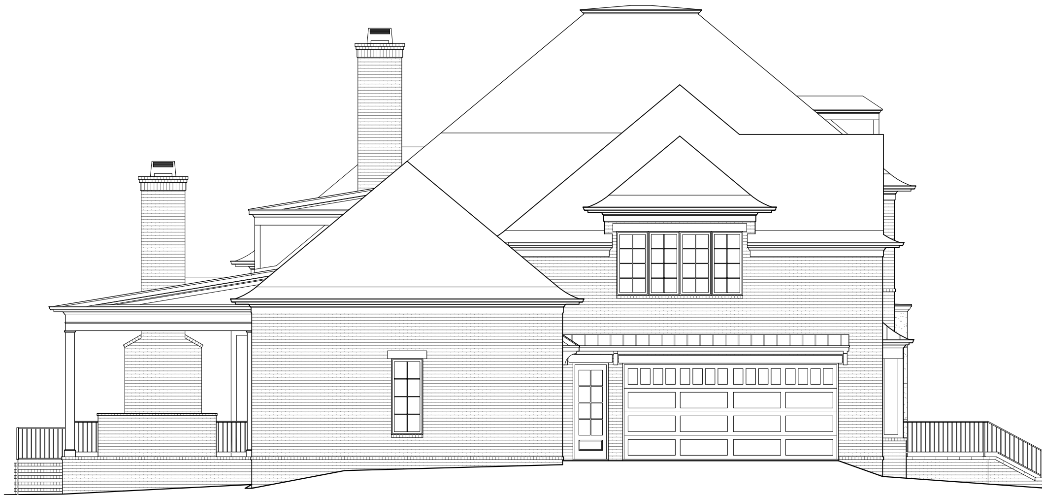
1 LEFT ELEVATION 1/8" = 1'-0"
