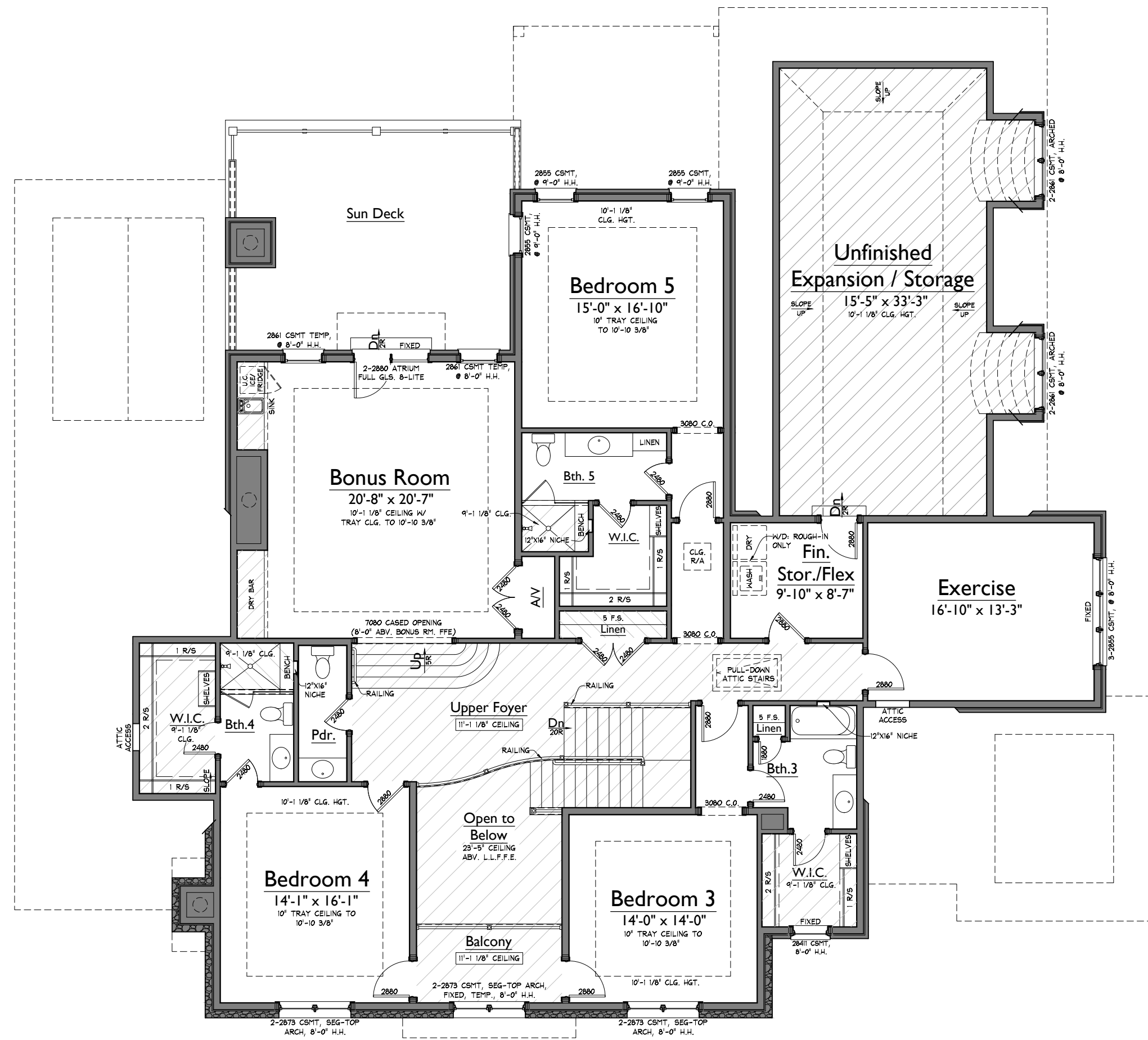
1 UPPER LEVEL FLOOR PLAN 1/8" = 1'-0"
