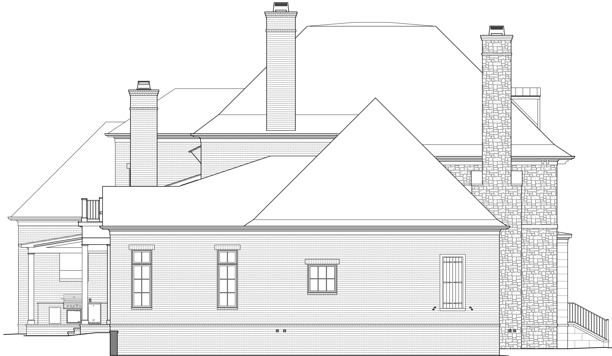
1 LEFT ELEVATION 1/8" = 1'-0"
