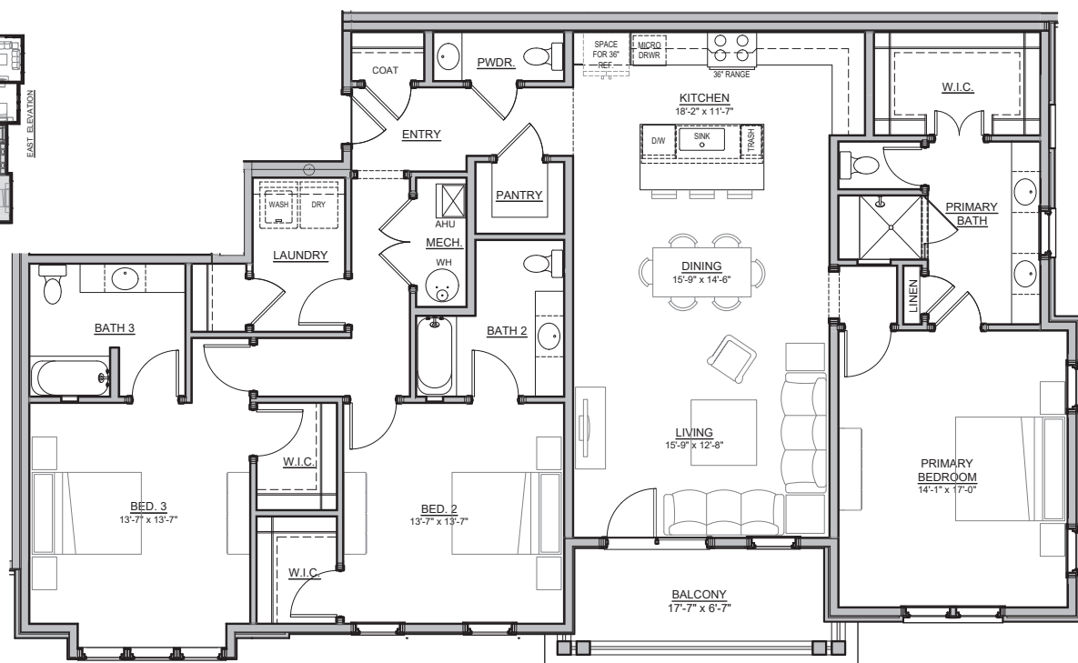
Floor Plan
